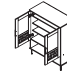
SC 55094-085 L800 X W370 X H1000 (MM) M3: 0.062 KG: 27.00 37-665-99
