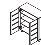
SC 335 WHITE/WG L800 X W335 X H890 (MM) M3: 0.054 KG: 22.00 37-600.4-50
