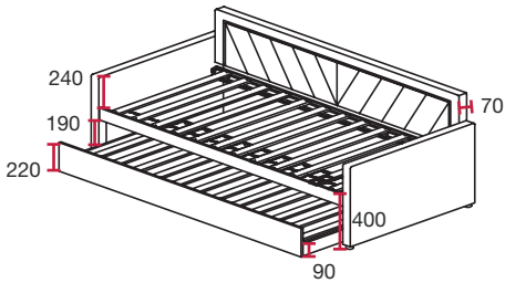
BR 11055-746 L2060 X W995 X H835 (MM) INNER (UP) : L1925 X W900 (MM) INNER (DOWN) : L1900 X W910 (MM) M3: 0.240 KG: 51.40 76-2280-65
