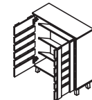
SC 55022-063 L800 X W315 X H920 (MM) M3: 0.062 KG: 25.40 86-589-92
